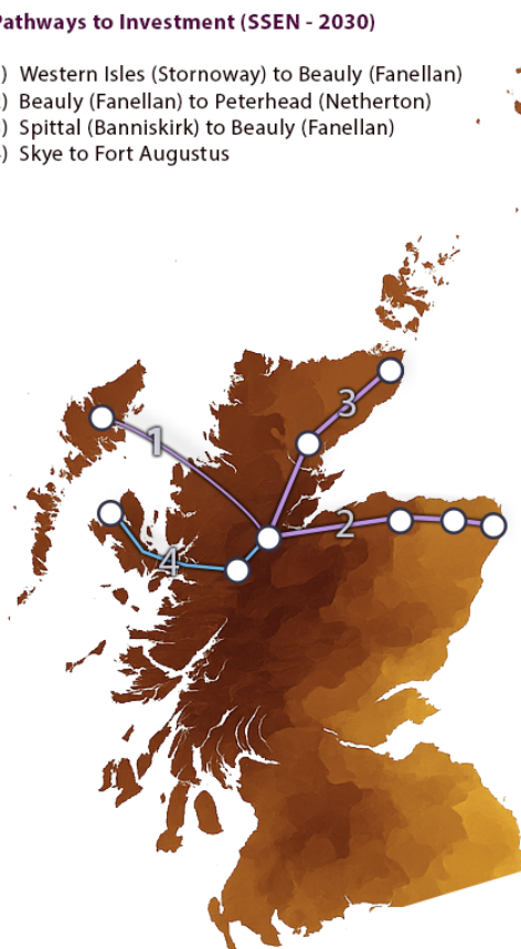
Fig: 1.2 Spatial visualisation of Chernobyl fallout over Great Britain in May 1986 (137 Cs activity (Bq/kg 1 Dry Matter ,DM). Copyright © NERC(CEH)2014. Overlaid with Pathways to Investment (SSEN -2030 Mapping Data).
