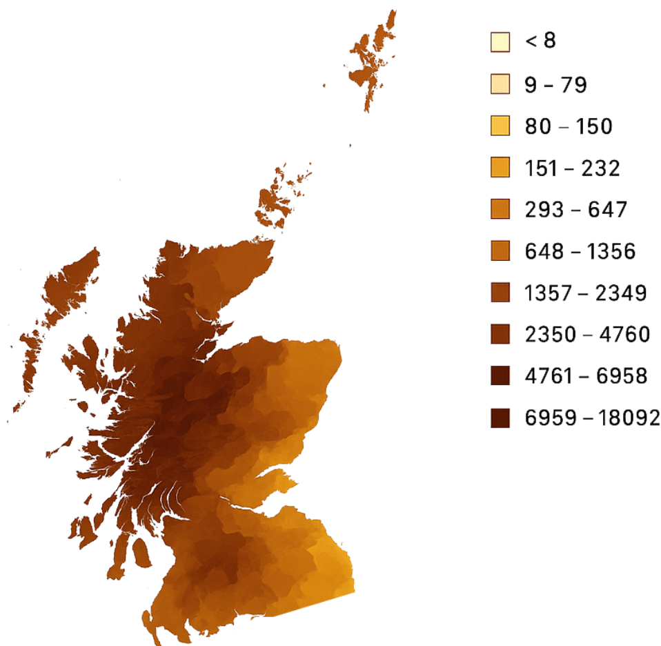
Fig: 1.1 Spatial visualisation of Chernobyl fallout over Scotland in May 1986 (137Cs activity 142 concentrations (Bq kg 1 Dry Matter ,DM). Extracted from Full United Kingdom Map. Copyright ©NERC (CEH) 2014.
