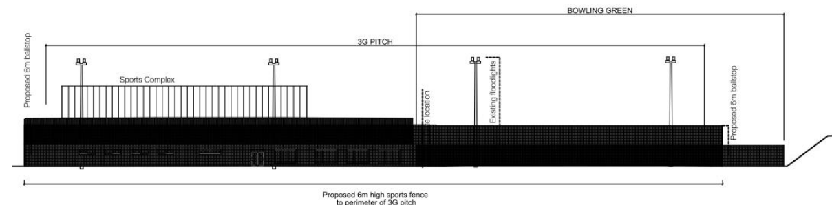
PROPOSED ELEVATION 04
