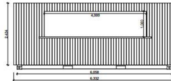
20ft Shipping Container - Side Elevation
