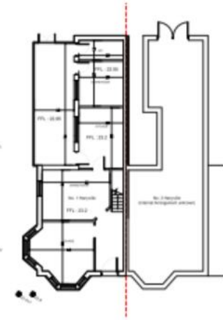
Existing Ground Floor Plan Relationship to existing openings to rear of adjacent dwelling
