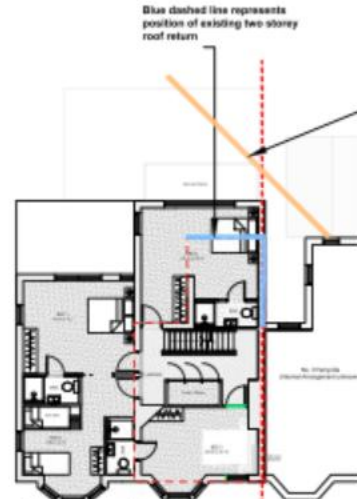
Proposed First Floor Plan Relationship to existing openings to rear of adjacent dwelling
