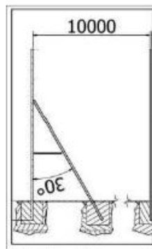
Fig. End post with support
